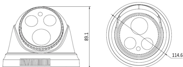
Installation Diagram
